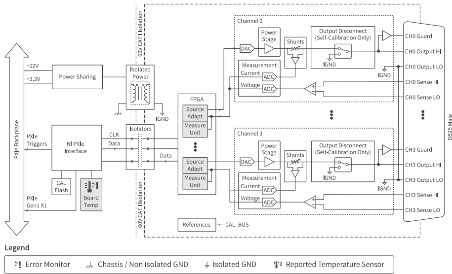
Figure 3. PXIe-4144 Channel-Level Block Diagram
