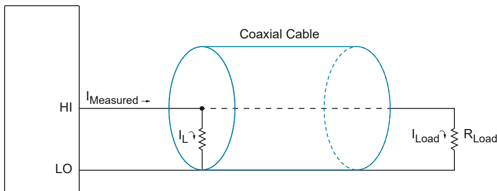
Figure 14. Leakage without Guarding ( I_{\text{Measured}} = I_{\text{Load}} + I_L )
