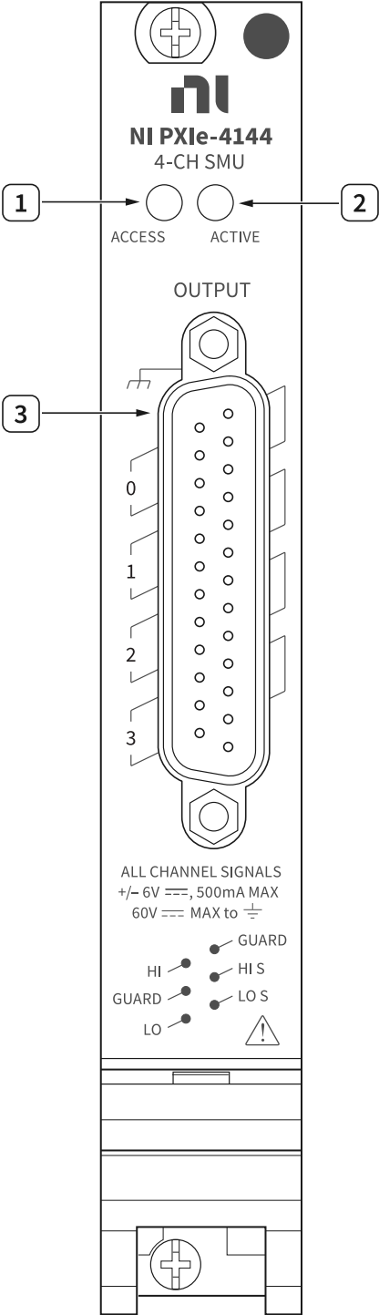
Figure 4. PXIe-4144 Front Panel
