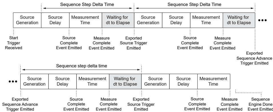
Figure 21. Sequence Step Delta Time in NI-DCPower Sequences
