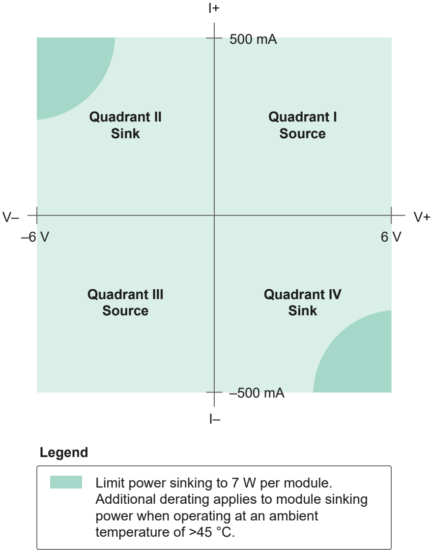
Figure 1. PXle-4144 Quadrant Diagram
