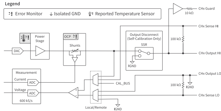
Figure 3. PXIe-4144 Channel-Level Block Diagram
