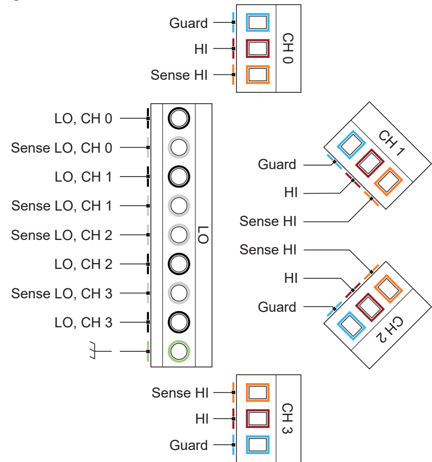
Figure 9. TB-414X Pinout
