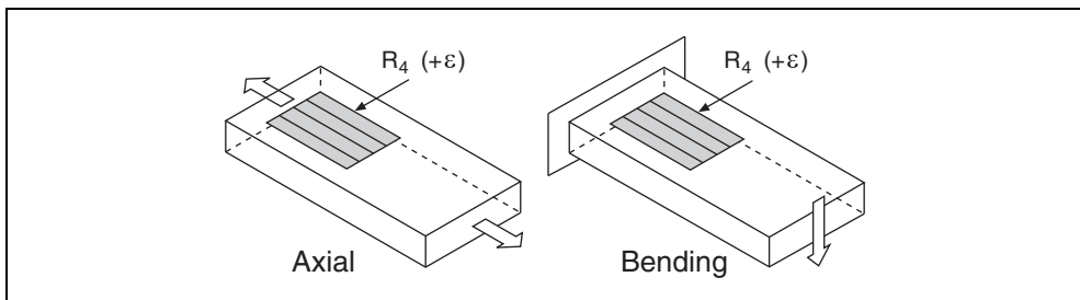
Figure 2-3. Quarter-Bridge Type I Measuring Axial and Bending Strain
