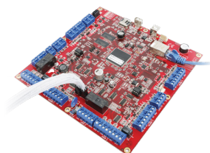
996035PCB&K Integriti IAC Controller PCB
